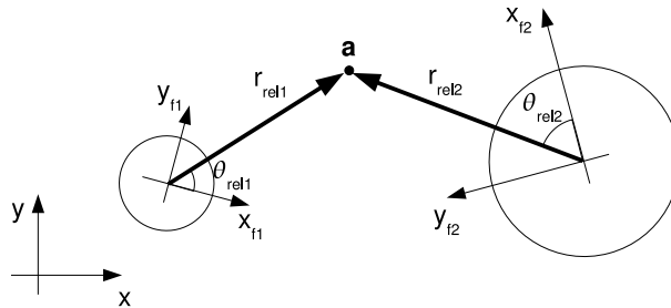
Fig. 2. The position of the anchor point is stored in the model as polar coordinates relative to the visual word scale and orientation.
