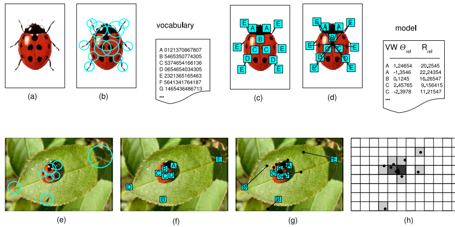
Fig. 1. Overview of the algorithm. Top row (model building): (a) model photo, (b) extracted local features, (c) features expressed as visual words from the vocabulary, (d) model description with relative anchor positions for each visual word. Bottom row (matching): (e) query image with extracted features, (f) visual words from the vocabulary, (g) anchor position voting based on relative anchor position, (h) Hough voting space.
